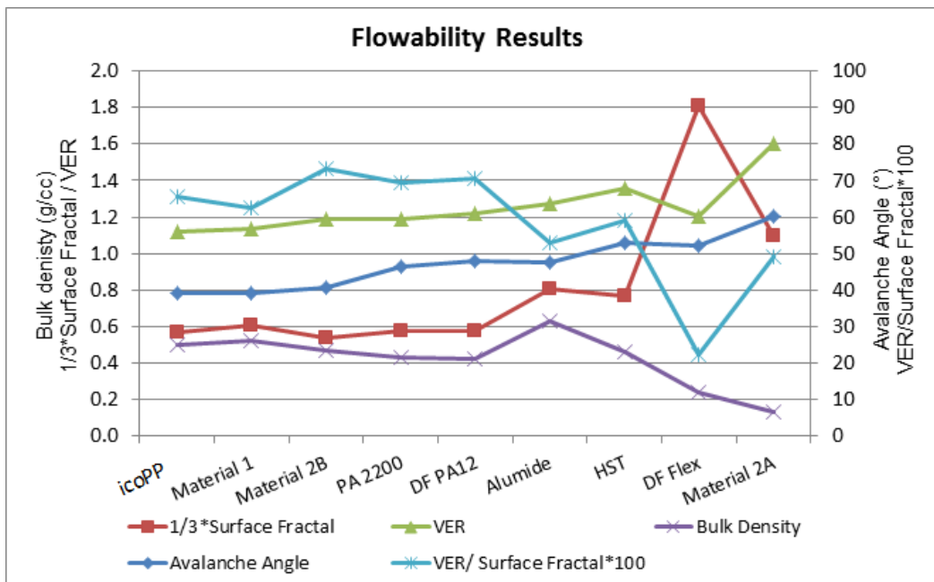
Figure 6: Summary of results for Flowability Indexes
