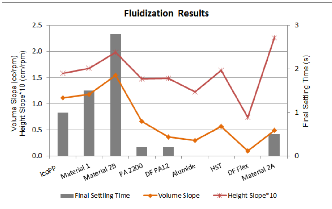
Figure 9: Summary of results for Fluidization Indexes
