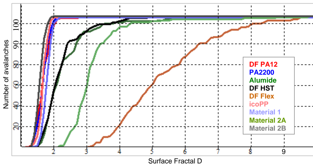
Figure 5: Cumulative Surface Fractal Distribution
