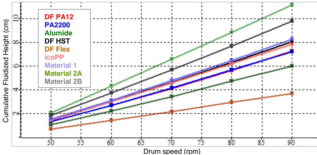
Figure 7: Cumulative Fluidized Height
