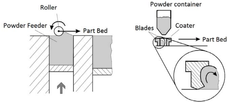
Figure 2: SLS powder spreading systems: Roller (3DSystems) & Blade (EOS) [28]
