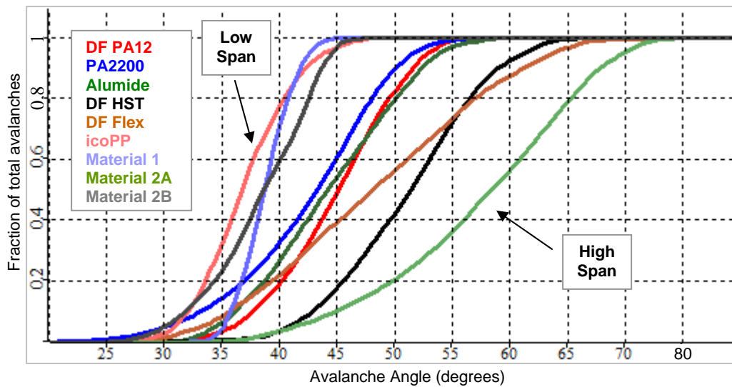
Figure 4: Cumulative Avalanche Angle Distribution
