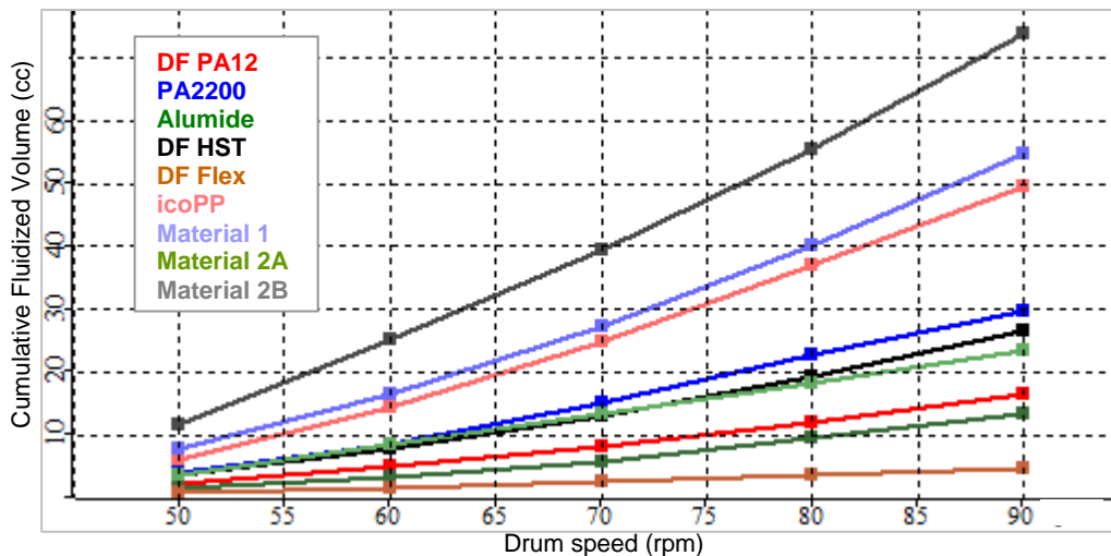
Figure 8: Cumulative Fluidized Volume
