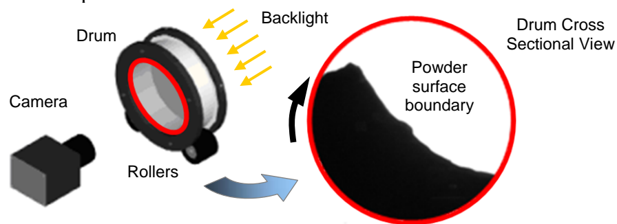
Figure 1: Schematic diagram of rotating and image acquisition system
