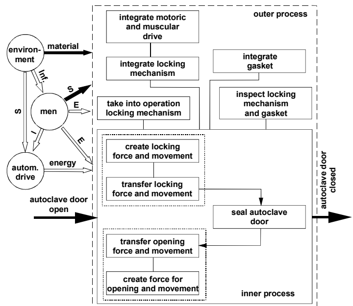
Figure 8. Example of a processual functional structure of an autoclave door, generated out of Figure 9 [8]
