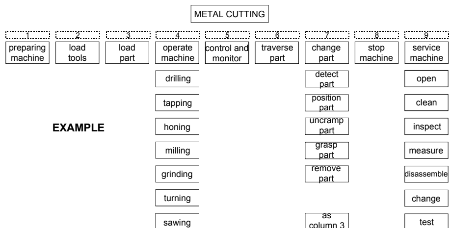
Figure 17. Hierarchical functional diagram of the machine tool from Figure 15 (from: Breiing, Mikron)
