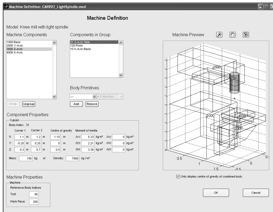
Fig. 2. Definition of the machine configuration for the Axis Construction Kit
