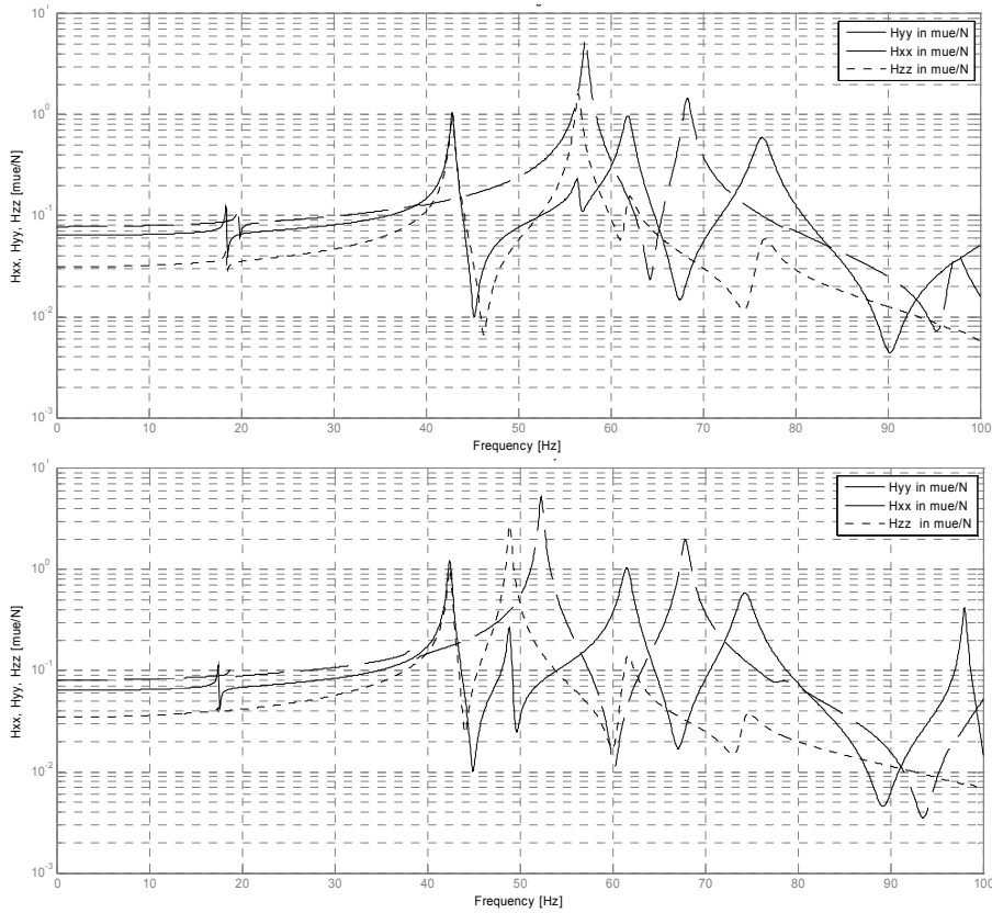
Fig. 4. Eigenfrequencies of the light (above) and heavy (below) variant under process loads
