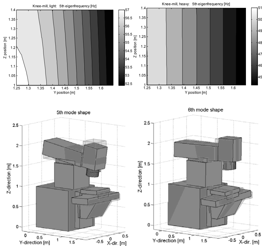
Fig. 3. Above: Distribution of 5th eigenfrequency for light (left) and heavy (right) spindle unit variant. Below: Mode shapes of the 5 th (left) and 6 th (right) mode (visualisation for the variant with heavy spindle unit)
