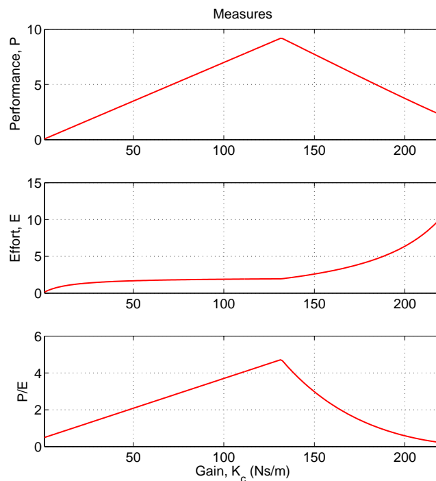
Figure 4: Measures obtained with the direct velocity feedback.
