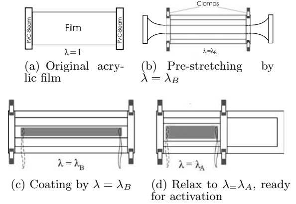
Figure 2: Schematic of the pre-stretching process
