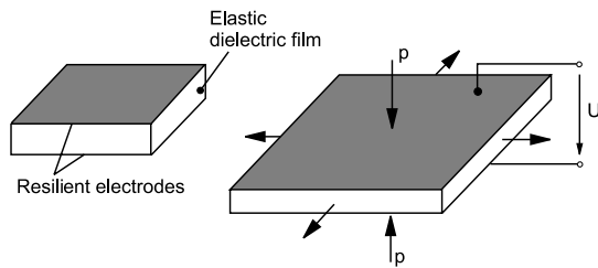
Figure 1: Simple working principle of an EAP
