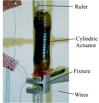
Figure 7: Measurement set-up of the cylindric dielectric polymer actuator
