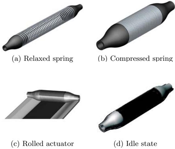
Figure 6: Schematic of cylindric dielectric polymer actuator
