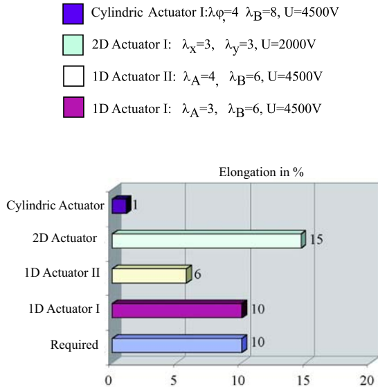
Figure 8: Elongation of the actuators in %
