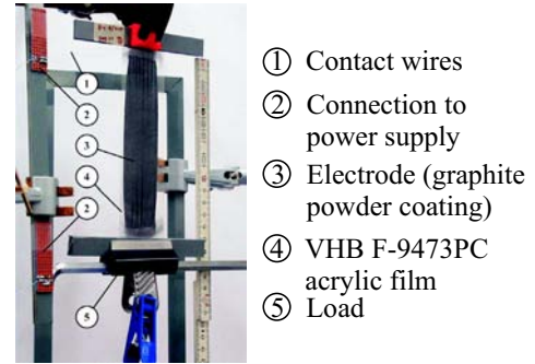
Figure 3: One-dimensionally pre-stretched flat polymer actuator
