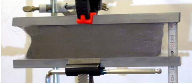
Figure 5: Two-dimensionally pre-stretched flat polymer actuator
