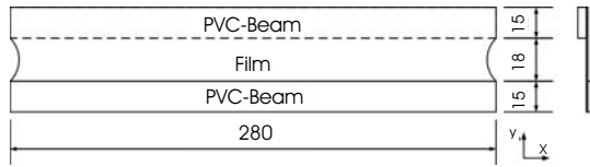
(a) Schematics of the actuator
