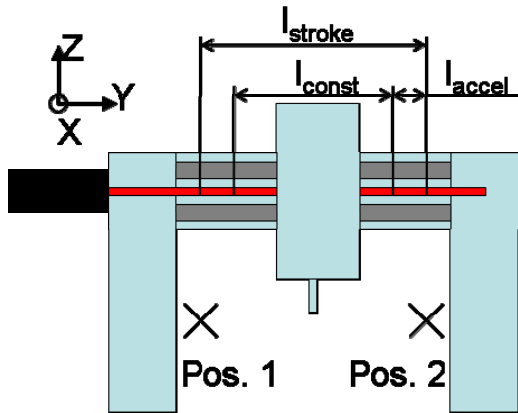
FIGURE 3. y-axis ball screw, Pos.1 and Pos.2: measurement positions.
