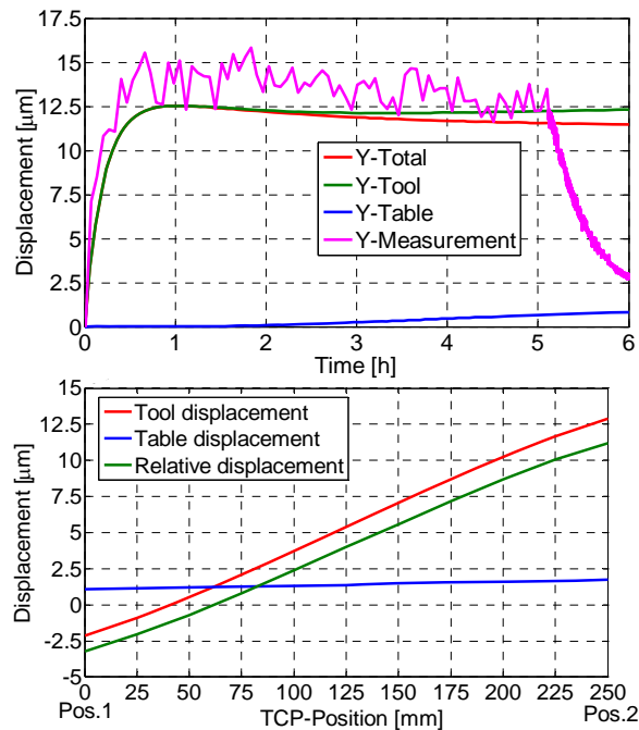
FIGURE 5. top: y-direction TCP-displacement in Pos.2, simulation and measurement, bottom: y-direction TCP-displacement for a virtual movement along the y-axis, Y-tool/YTable: TCP-displacement on the tool/table side.
