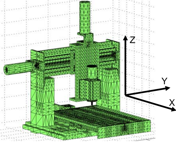
FIGURE 1. Model of the three axes machine tool with about 5'000 elements.
