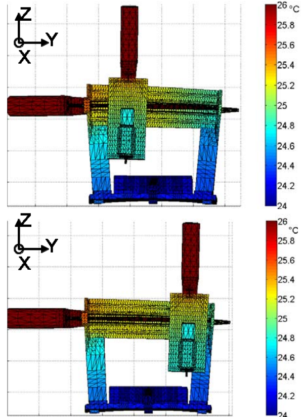
FIGURE 4. Simulation results: Temperature distribution and deformation, scale factor 10'000, steady state, top: Pos. 1, bottom: Pos.2.
