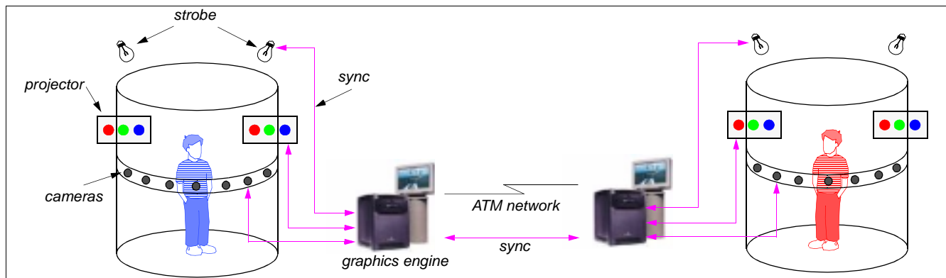
Figure 1: Schematic setup of the Blue-C. environment.
